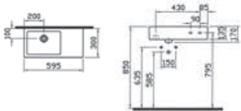
Technical drawing shows right hand shelf 0TH basin only
