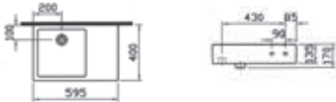
Technical drawing shows right hand shelf 0TH basin only
