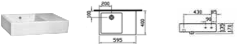
Technical drawing shows right hand shelf 0TH basin only
